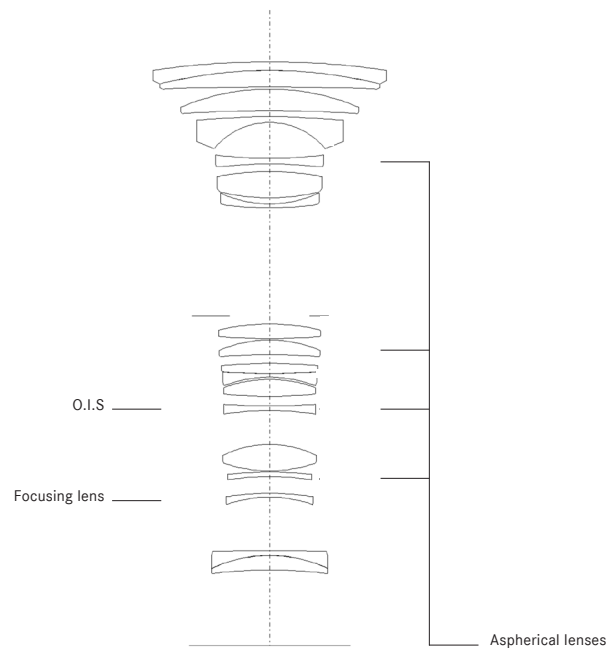
LENS SHAPE
